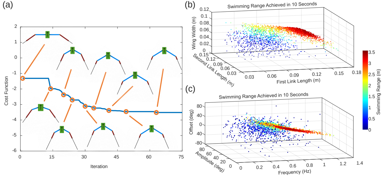
Fig. 5: Design optimization using the dynamic model. (a) The value of optimization cost function and the evolution of the robot design. Feasible parameter sets in the optimization process: (b) Fin system design parameters and (c) input gaits.
