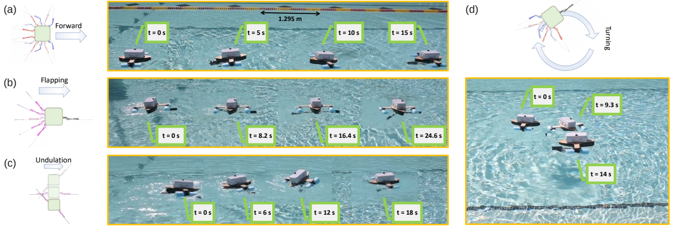
Fig. 7: Untethered robot swimming. (a) Swimming forward using rowing gaits of both fins. (b) Swimming laterally using one fin flapping actuation. (c) Swimming using undulating gait. (d) Turning by rowing gaits of one fin.
