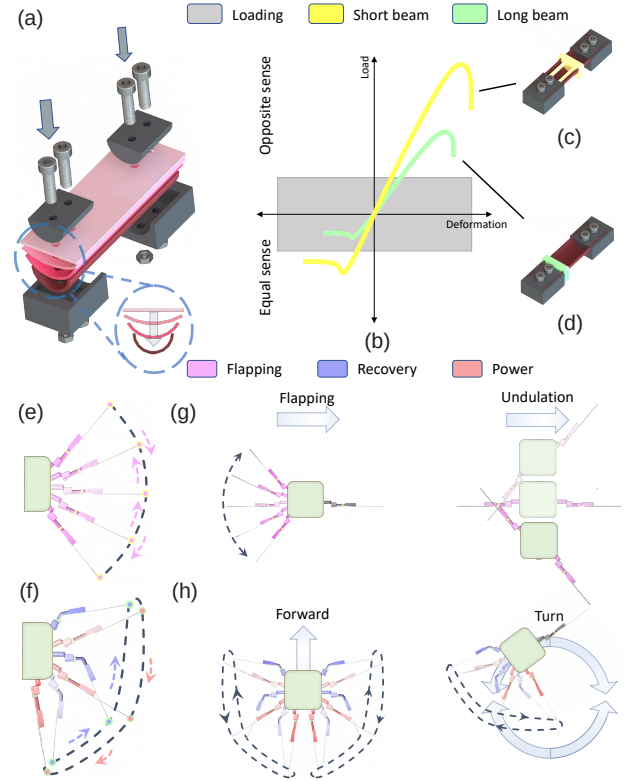
Fig. 1: Utilizing curved beams in rowing and flapping swimming strategies. (a) Curving mechanism. (b) The nonlinear behavior of curved beams. (c) short beam. (d) long beam. (e) flapping gait. (f) Rowing gait. (g) Lateral swimming using one fin flapping gait, and undulation. (h) Forward swimming and turning using rowing gait.
